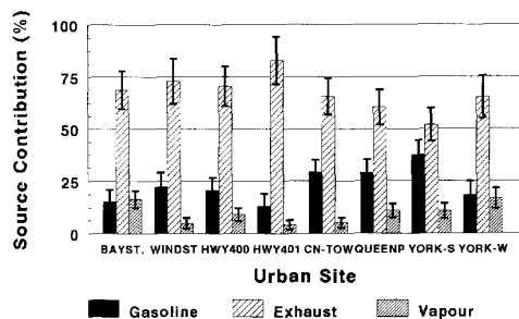
Fig. 4. Contributions of sources to gasoline based NMHCs calculated by the chemical mass balance model at urban sites in Toronto. Bay St., Windsor Tunnel, Hwy 400 and Hwy 401 are roadside sites, CN-Tower and Queen's Park are non-roadside downtown sites. Calculations were made for the York University site by sectoring observations to summer (S) and winter (W) seasons.
