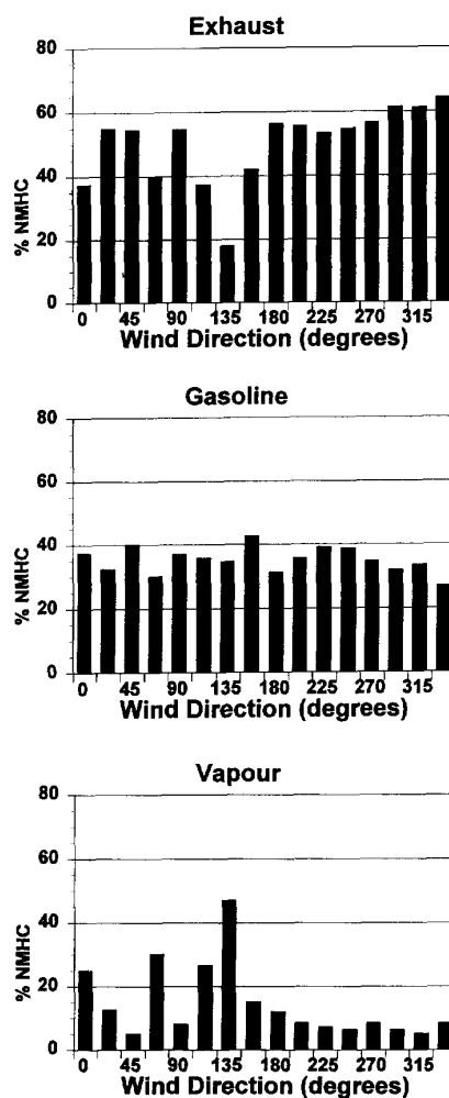
Fig. 5. Relative contributions of sources to gasoline based NMHCs at York University (summer 1991–92) calculated by the chemical mass balance model. Results were calculated for data sets sectoring by wind source direction where 0° is north, 90° is east.
