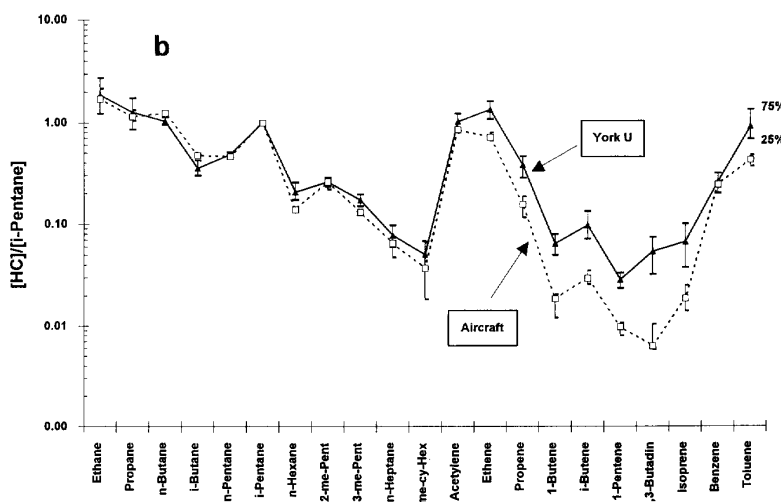
Fig. 3b. Comparison of hydrocarbon distributions recorded at York University (ground level) and by aircraft measurements above Toronto during SONTOS.
