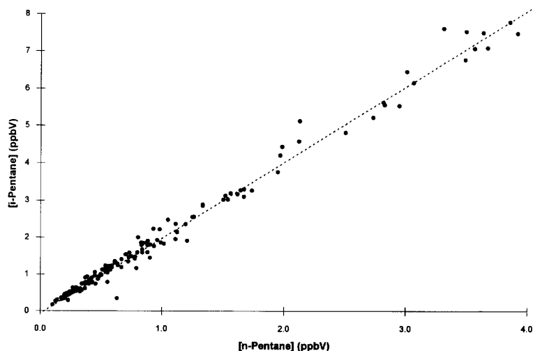
Fig. 2. Linear correlation between isopentane and n -pentane for observations made at York University during the summer of 1992. Slope = 2.03 \pm 0.02 , Y-intercept = -0.02 \pm 0.02 , r = 0.99 .
