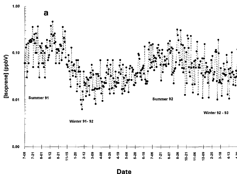
Fig. 6a. Seasonal distribution of isoprene mixing ratios at York University.
