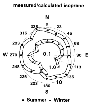
Fig. 7. Measured/calculated isoprene concentrations. Isoprene concentrations were calculated by the CMB model based upon the assumed 0.0018% NMHC mass assumed in the exhaust profile. The radial component represents the ratio which is presented on a log scale (0.1 centre to 10.0 outer ring).
