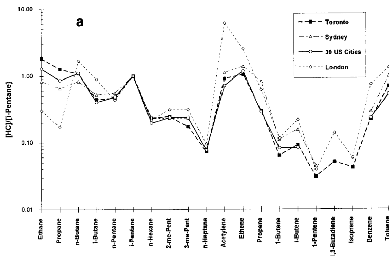
Fig. 3a. Comparison of urban hydrocarbon distributions at several cities with those measured at York University (Toronto).
