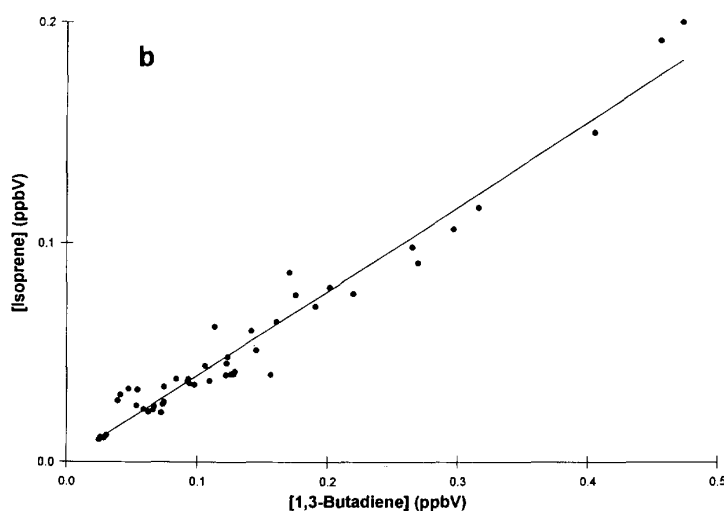
Fig. 6b. Linear correlation between isoprene and 1,3-butadiene for observations at York University during the winter of 1992. Slope = 0.38 \pm 0.02 , Y-intercept = 0.001 \pm 0.002 , r = 0.98 .
